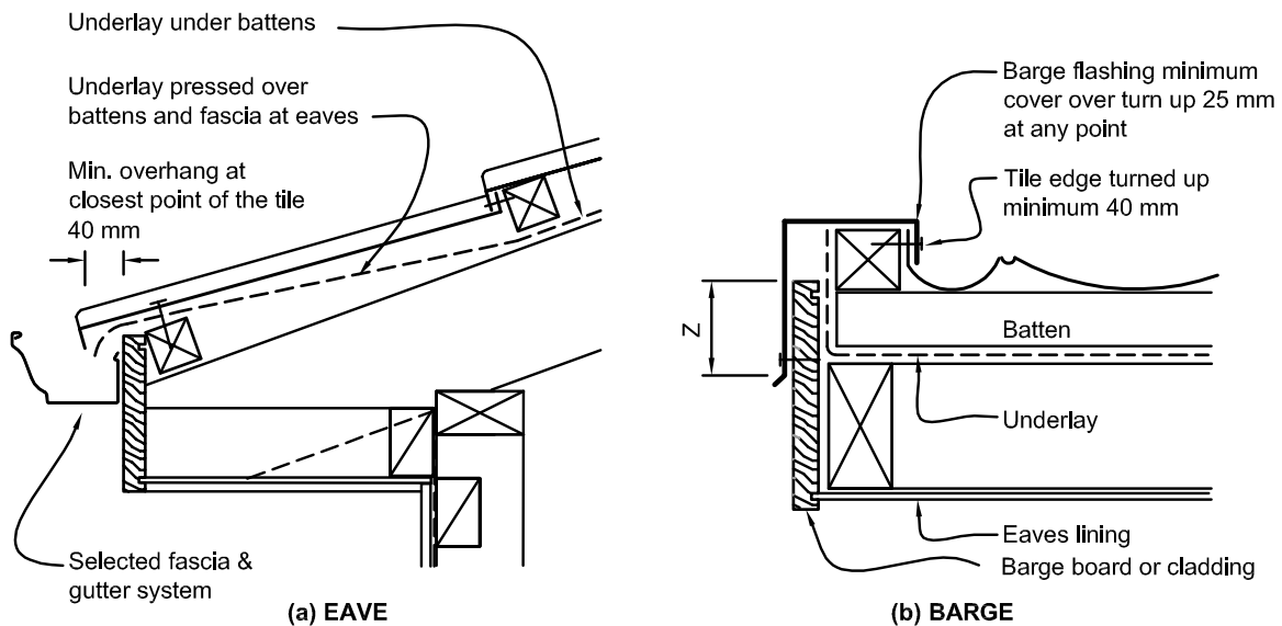
Figure 8.3.6.1C: Eaves and barges for metal tile
