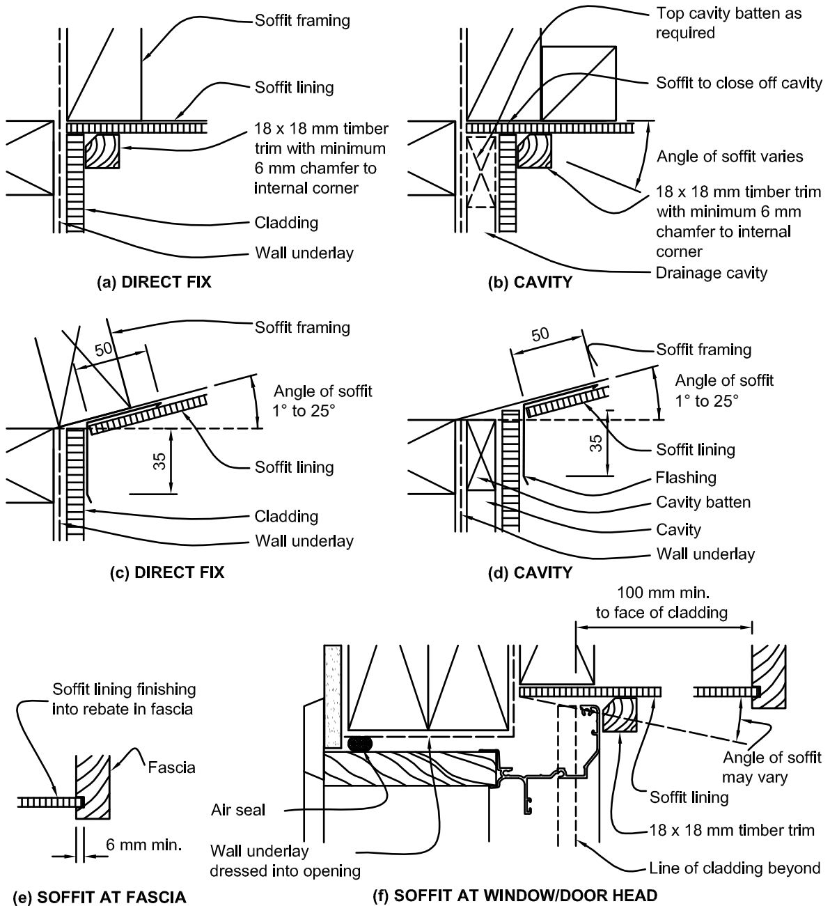
Figure 5.1.4.2: Soffit/wall junction
