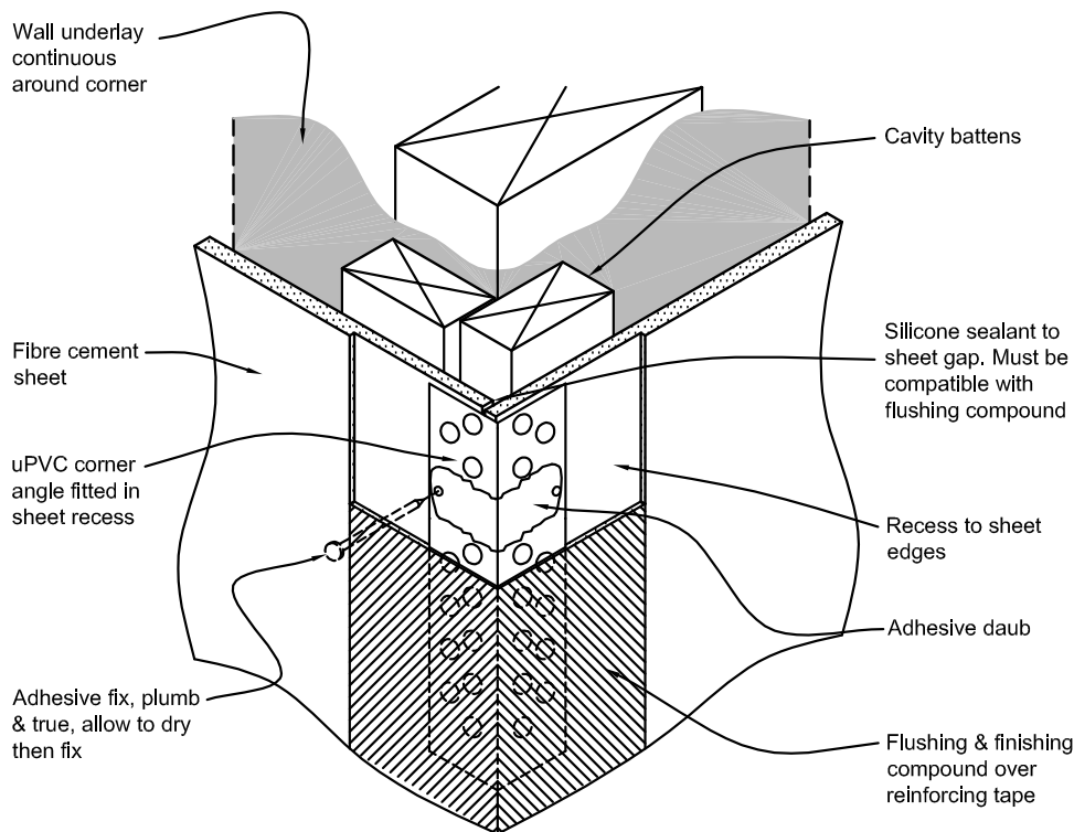
Figure 9.7.5.4: Flush-finished external corners for fibre cement sheet
