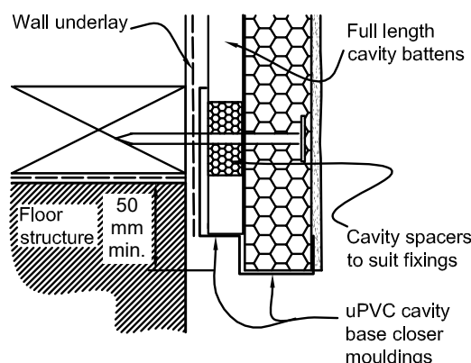
Figure 9.9.6.1: Bottom of cladding for EIFS
