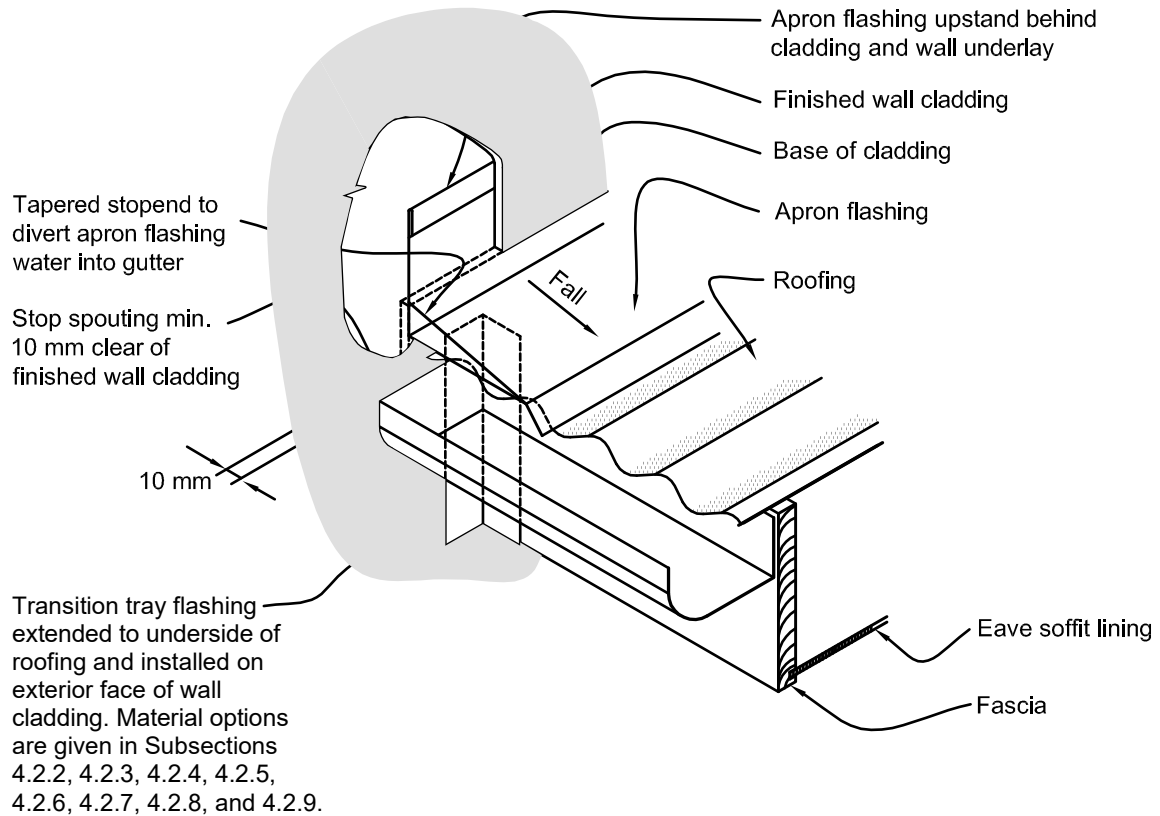
Figure 5.1.2.4: Gutter/wall junction
