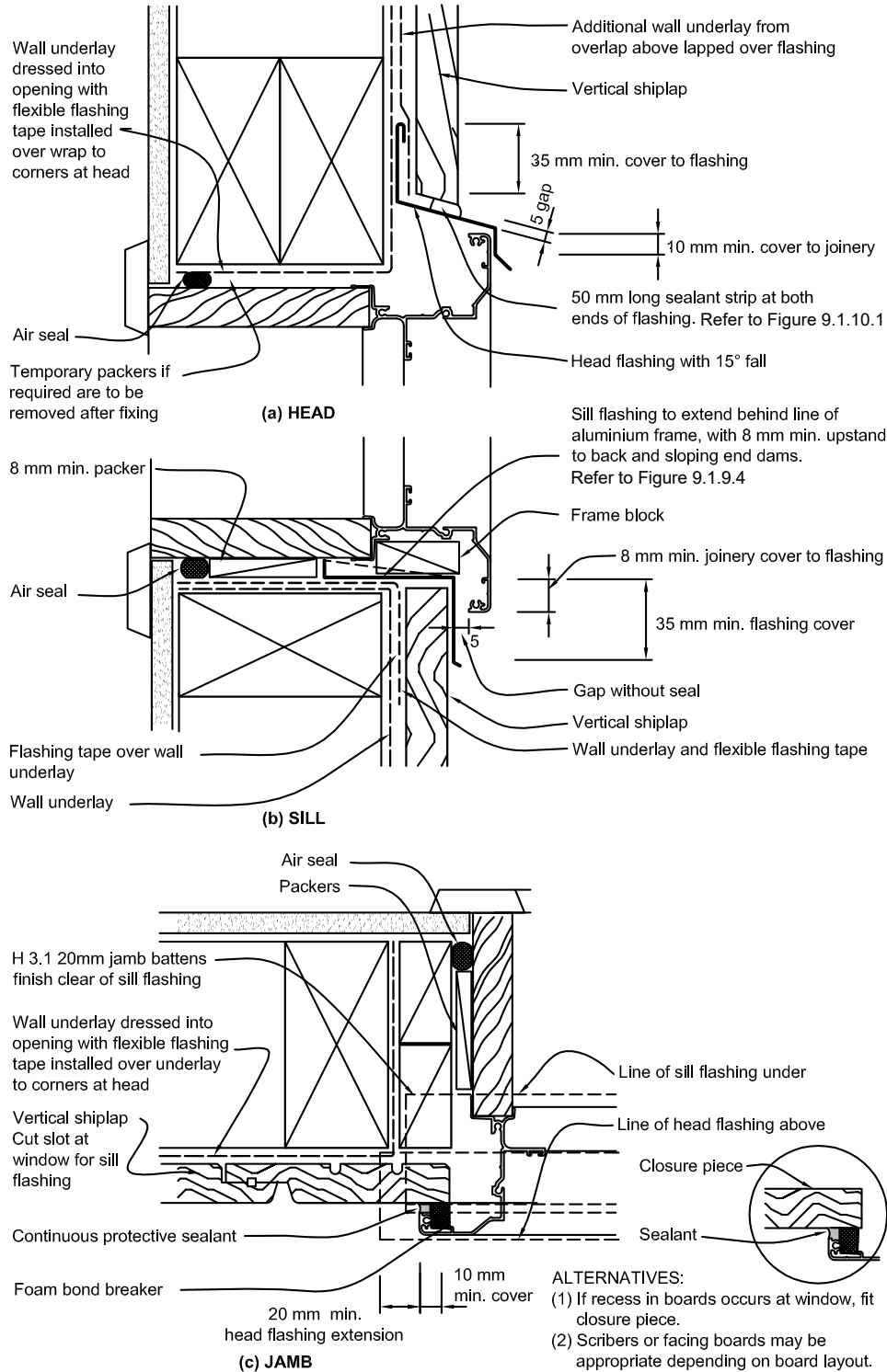
Figure 9.4.6.1C: Windows and doors for direct fixed vertical shiplap weatherboards Paragraph 9.4.6.1
