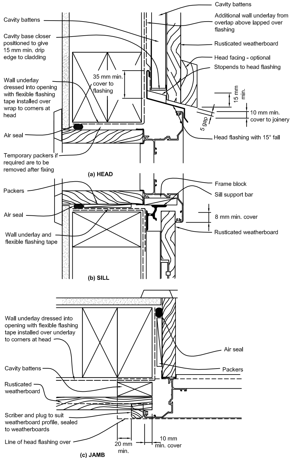
Figure 9.4.7.2: Windows and doors for rusticated weatherboards on cavity Paragraph 9.4.7.2
