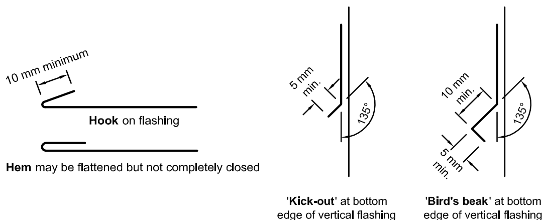
Figure 4.4.3.2: Typical metal flashing edge treatments
