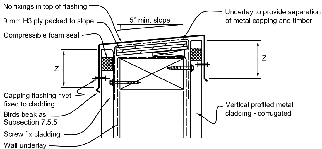
Figure 9.6.6.9: Balustrade and parapet for vertical profiled metal
