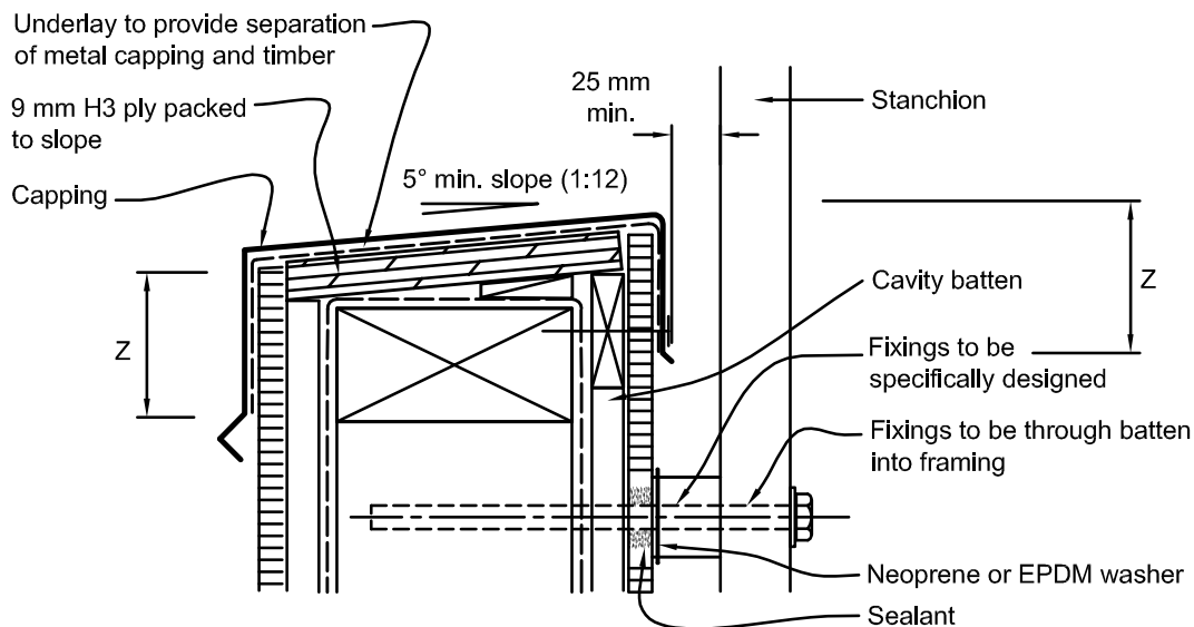
Figure 7.5.6.1: Stanchion fixing
