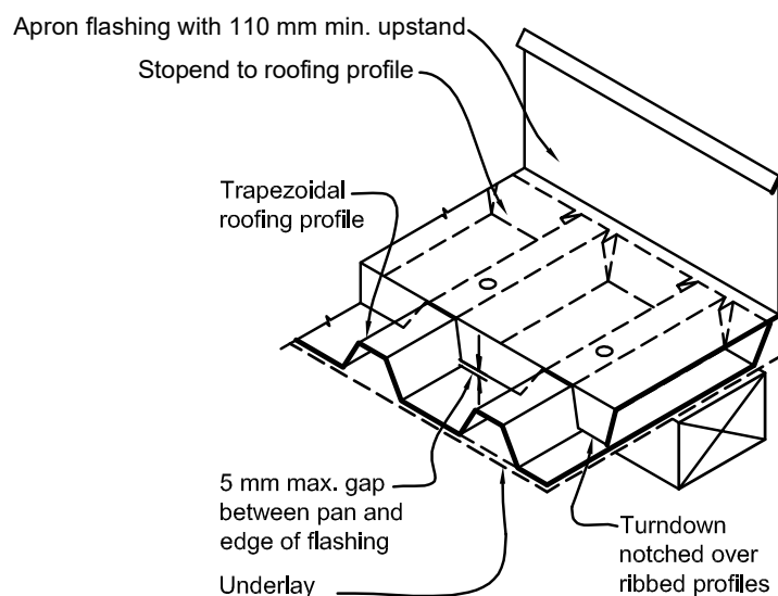
Figure 8.4.9.2B: Trapezoidal notched flashing
