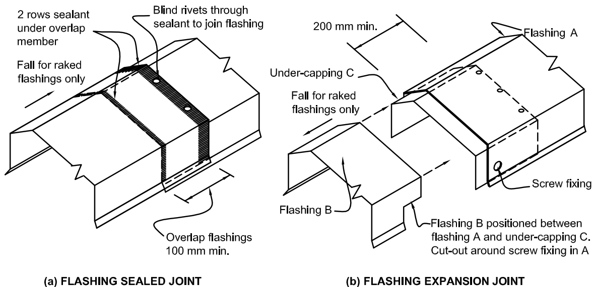
Figure 4.4.4.1: Joints in metal flashings
