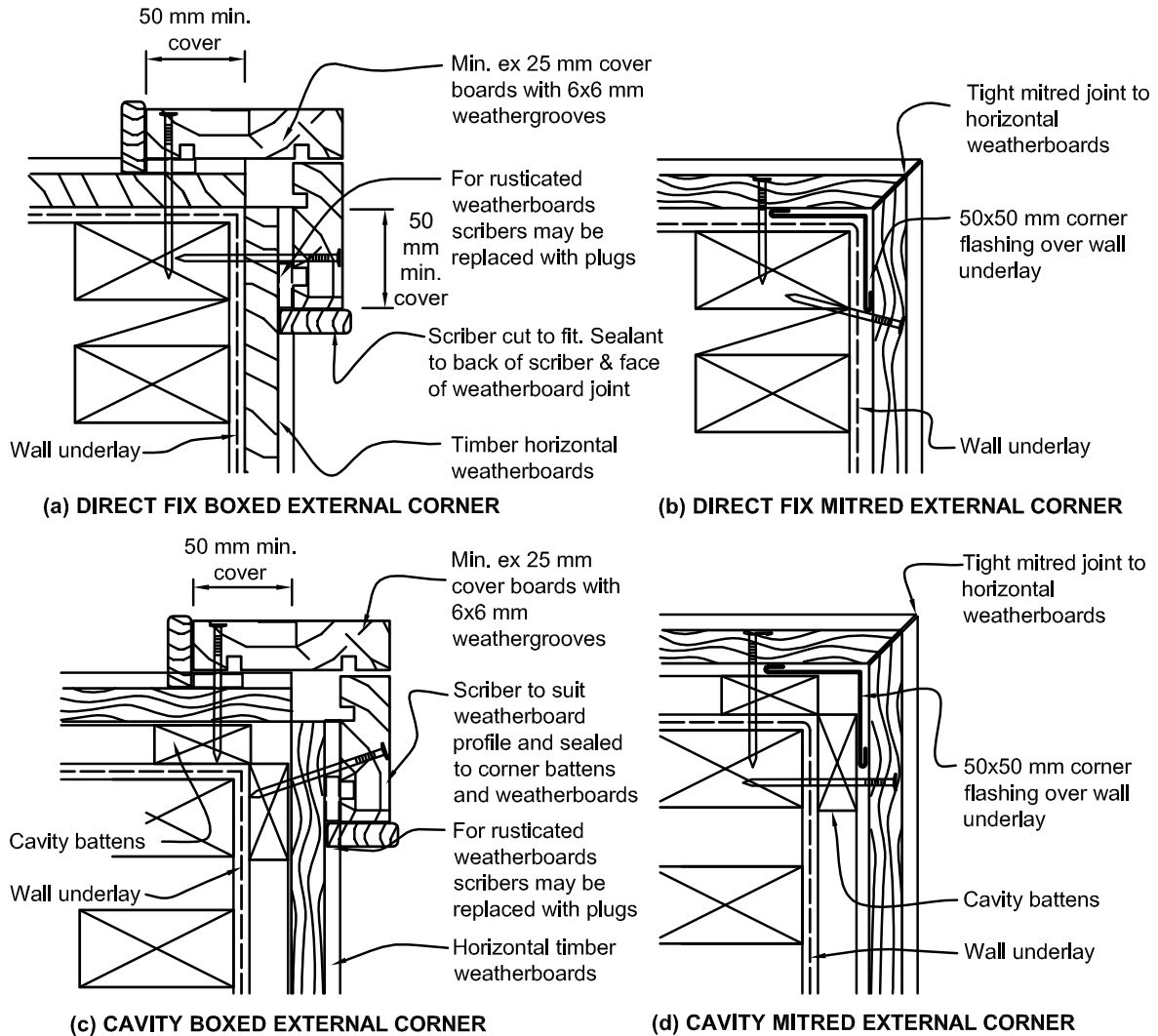
Figure 9.4.4.4B: External corners for horizontal weatherboards
