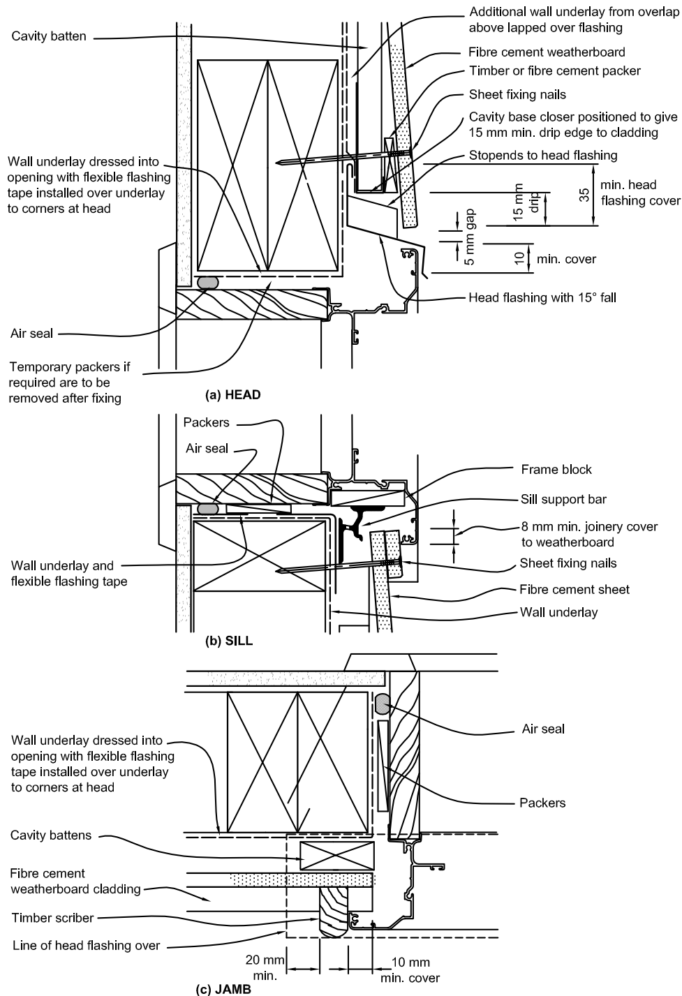
Figure 9.5.4.3: Windows and doors in fibre cement weatherboards on cavity
