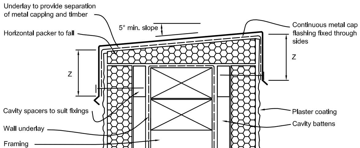
Figure 9.9.9.4: Parapet with metal capping for EIFS
