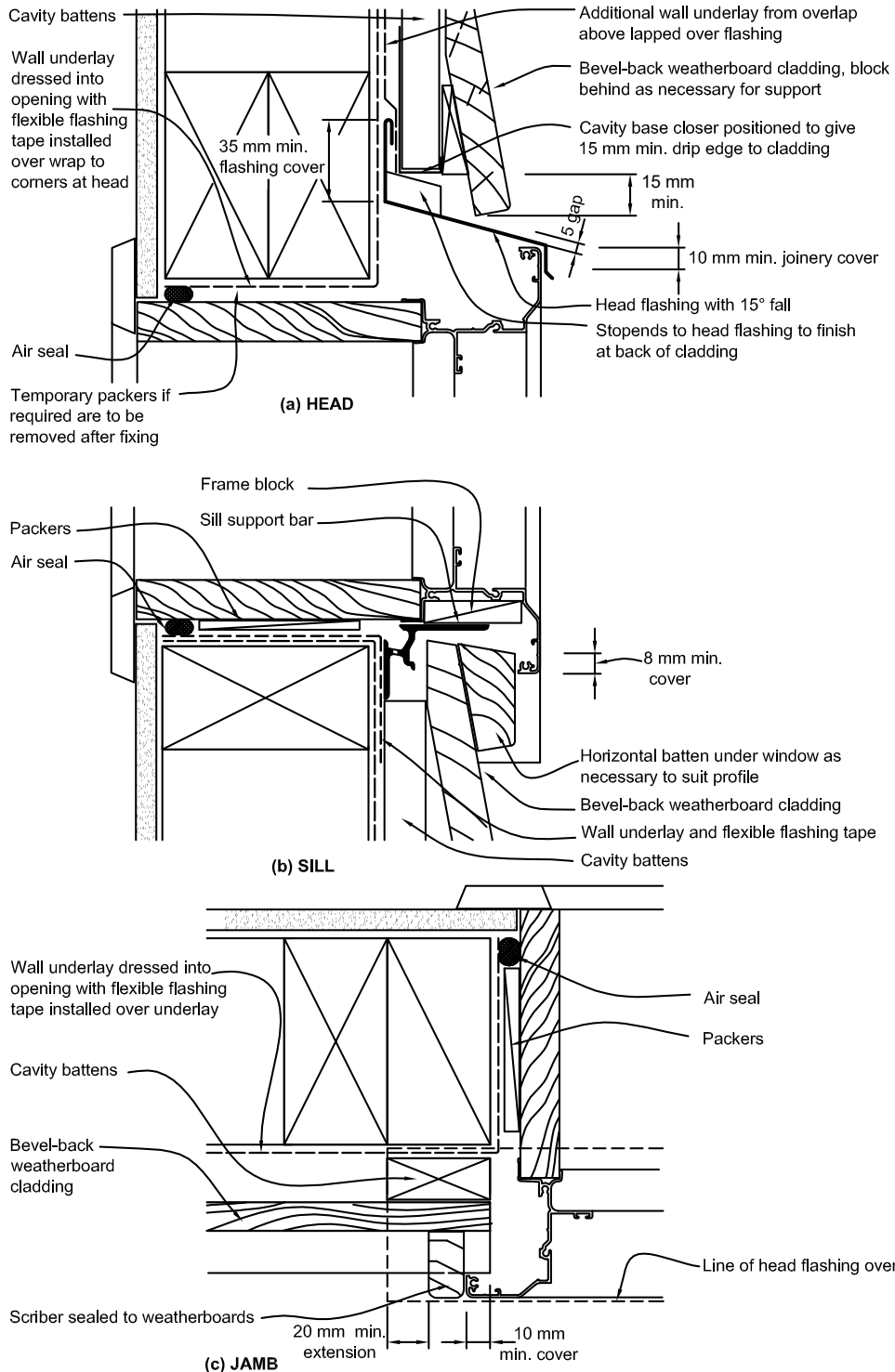
Figure 9.4.7.1: Windows and doors for bevel-back weatherboards on cavity
