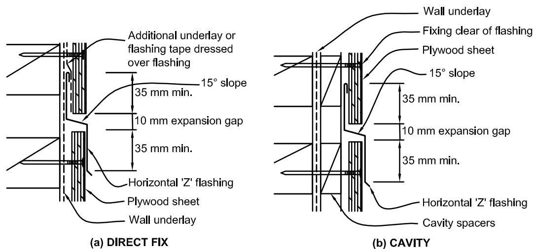
Figure 9.8.3.3: Horizontal joints for plywood sheet
