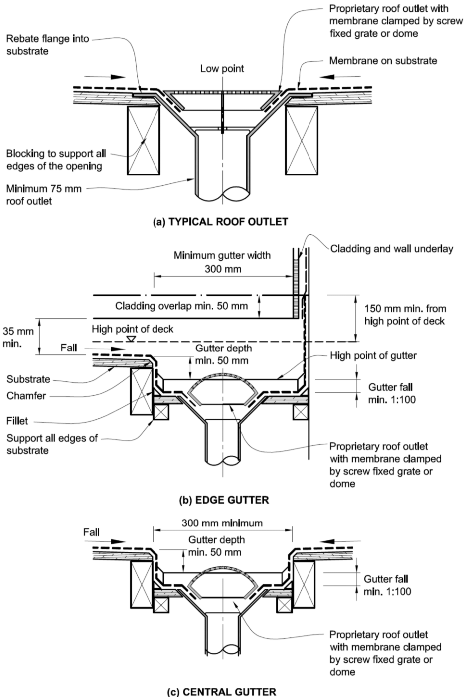
Figure 8.5.8.1: Gutters and outlets in membrane
