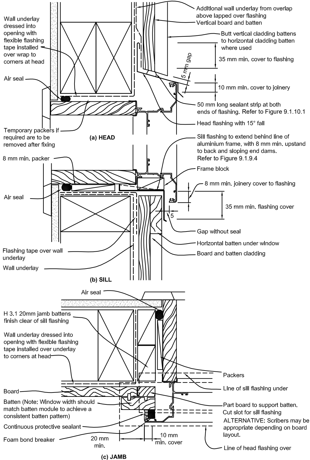
Figure 9.4.6.1D: Windows and doors for direct fixed board and batten weatherboards Paragraph 9.4.6.1
