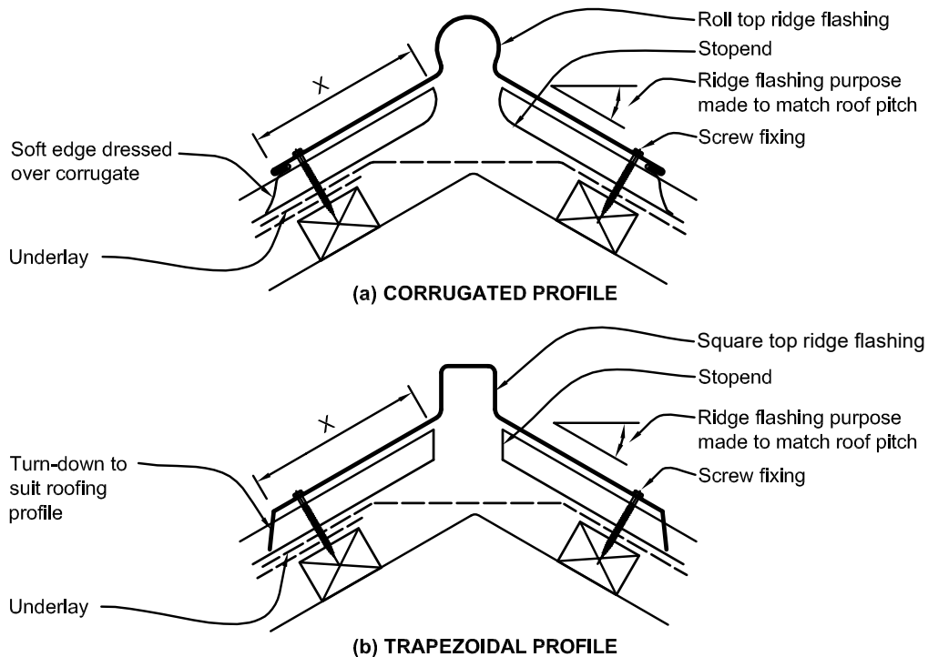
Figure 8.4.9.7D: Ridge and hip flashings for profiled metal
