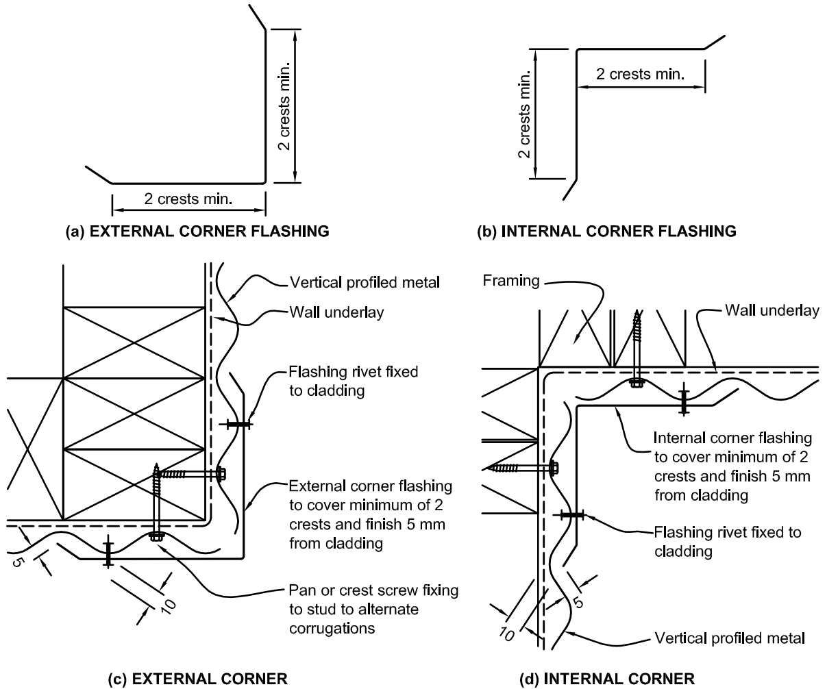
Figure 9.6.6.5: Corners for vertical profiled metal
