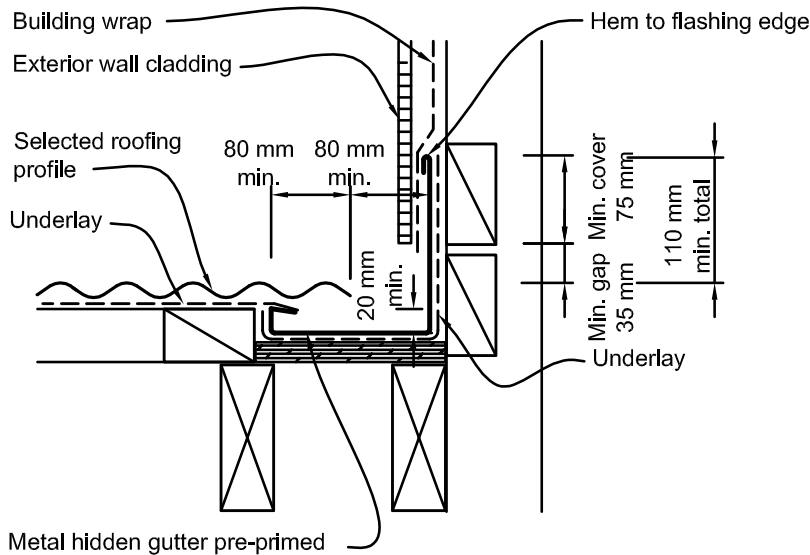
Figure 8.4.11.2: Parallel hidden gutter for profiled metal
