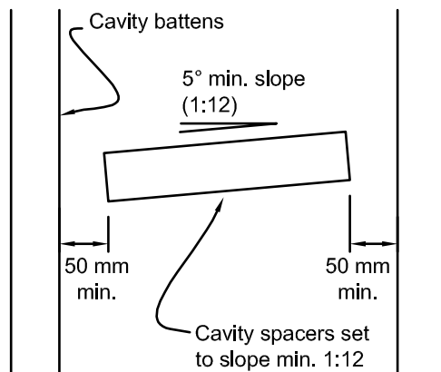
Figure 9.1.7.4B: Cavity spacers
