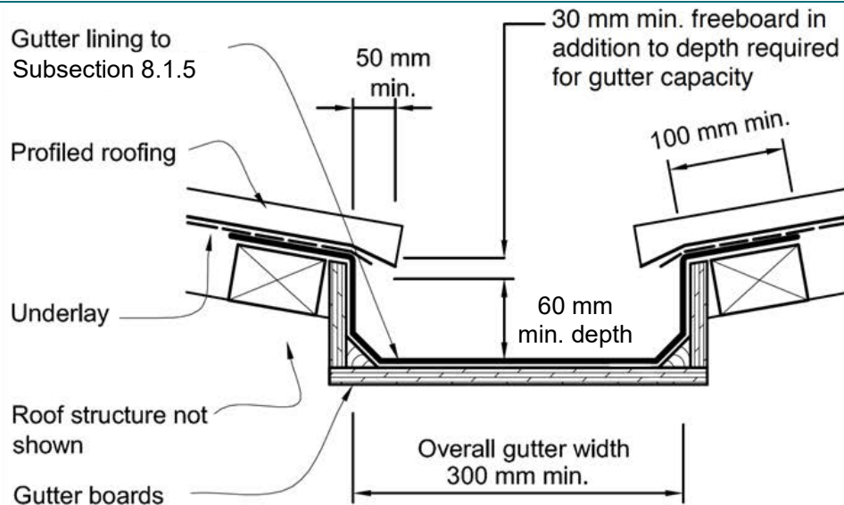
Figure 8.4.11.4: Internal gutter for profiled metal
