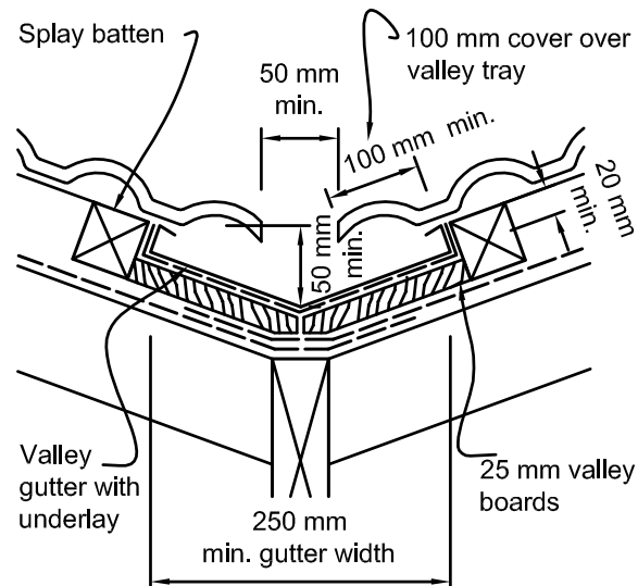
Figure 8.2.5.1E: Valley for masonry tile
