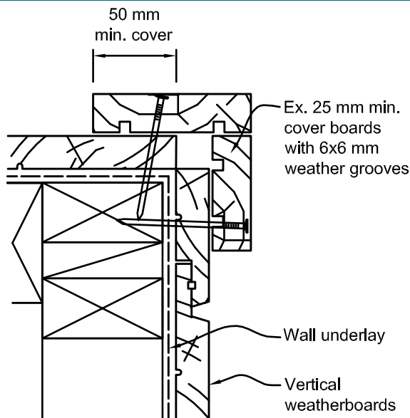
Figure 9.4.5.5: External corners for vertical weatherboards
