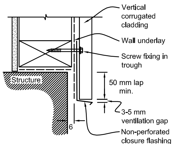
Figure 9.6.6.4: Bottom of cladding for vertical profiled metal
