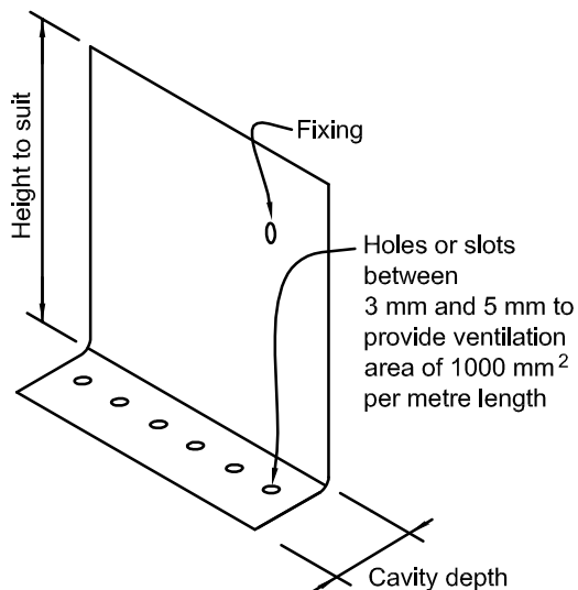
Figure 9.1.7.4A: Cavity base closer/vermin proofing
