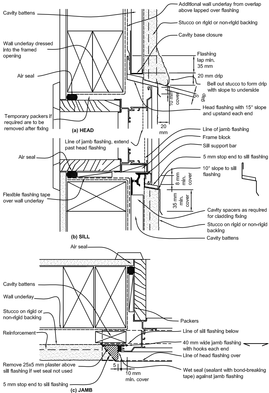
Figure 9.3.9.1: Windows and doors in stucco cladding Paragraph 9.3.9.1
