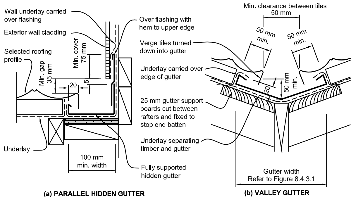
Figure 8.3.6.1D: Hidden gutter and valley gutter flashings to metal tile
