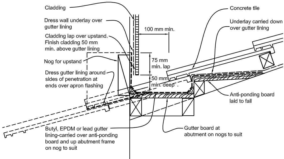
Figure 8.2.5.1I: Flashing to framed penetration for masonry tile
