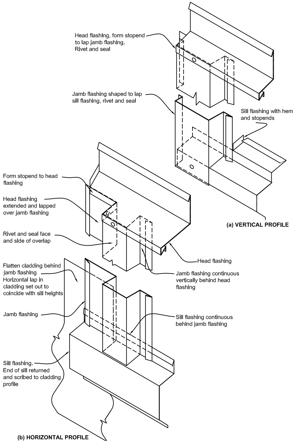
Figure 9.6.7.9B: Window and door flashings for profiled metal Paragraphs 9.6.6.8 and 9.6.7.9
