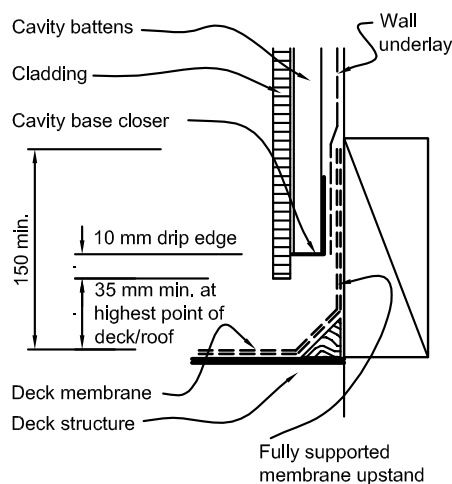
Figure 7.5.4.1: Enclosed balustrade – bottom of cladding
