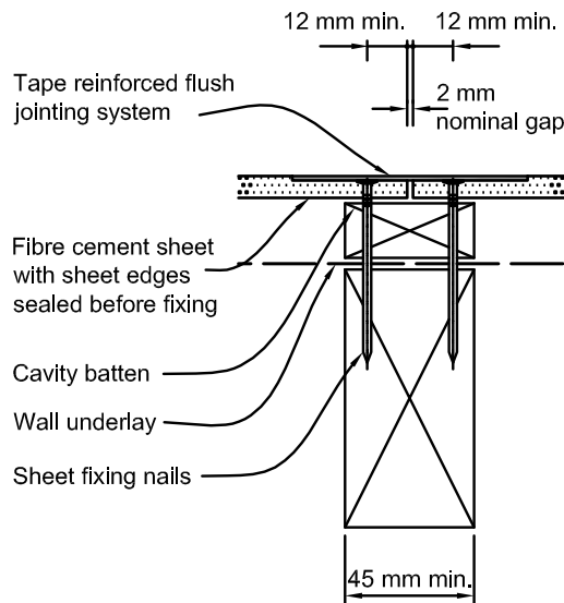
Figure 9.7.5.3: Flush-finished joints for fibre cement sheet
