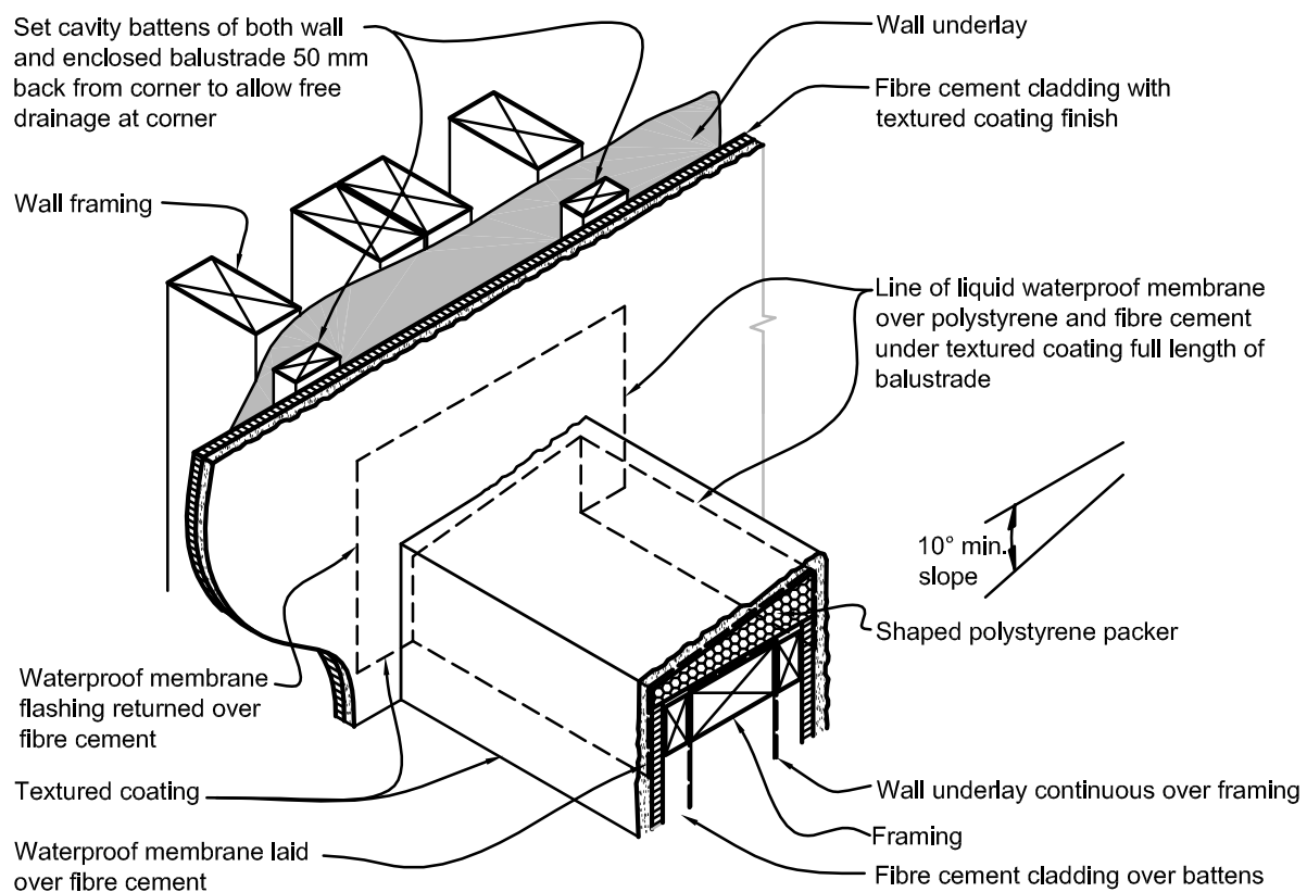
Figure 9.7.8.4: Enclosed balustrade to wall for fibre cement sheet
