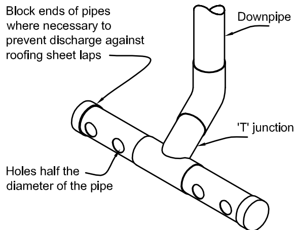
Figure 8.1.4.5: Spreader for roof discharge
