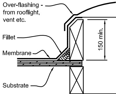
Figure 8.5.7.1A: Roofing penetration in membrane
