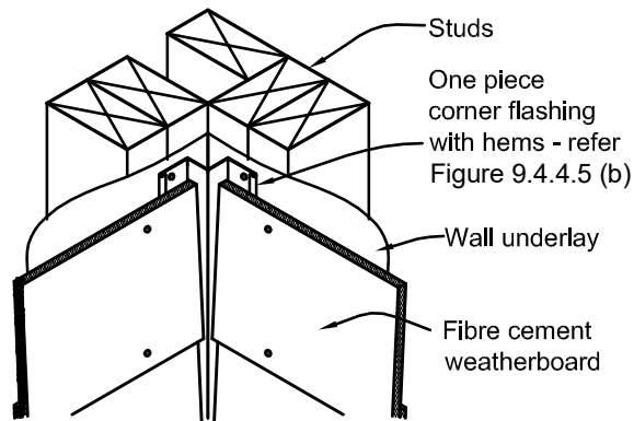
Figure 9.5.3.7: Aluminium corners in fibre cement weatherboards
