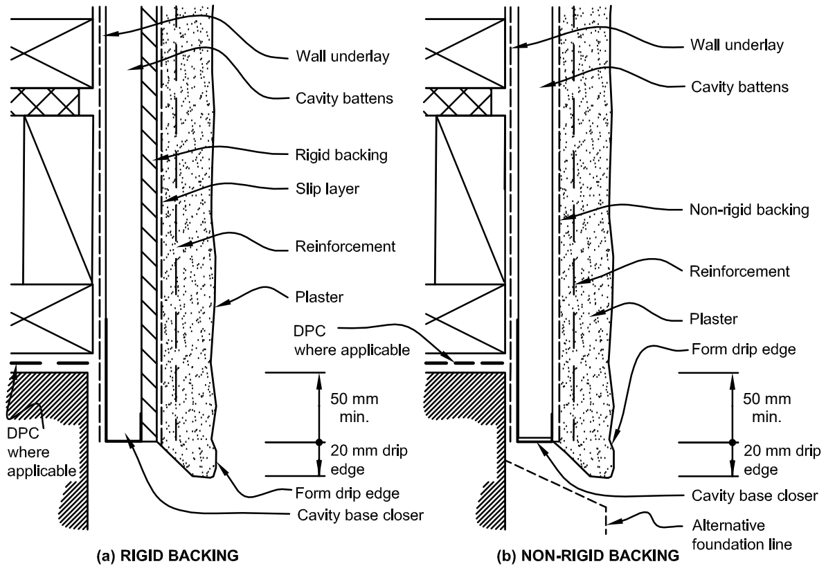
Figure 9.3.7.1: Bottom of stucco cladding
