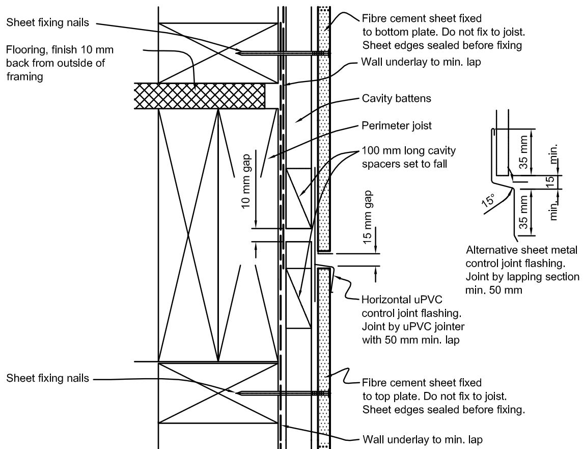
Figure 9.7.4.1E: Horizontal joints for fibre cement sheet on cavity
