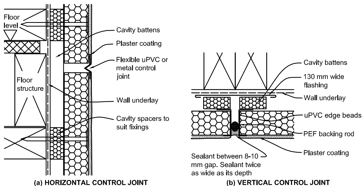
Figure 9.9.3.4: Control joints for EIFS
