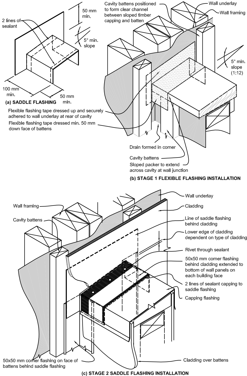
Figure 6.2.3.1B: General junction of parapet and enclosed balustrade-to-wall with metal capping (figure notes on next page)
