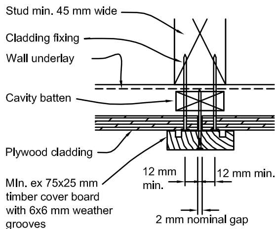
Figure 9.8.2.1: Battened joints for plywood sheet
