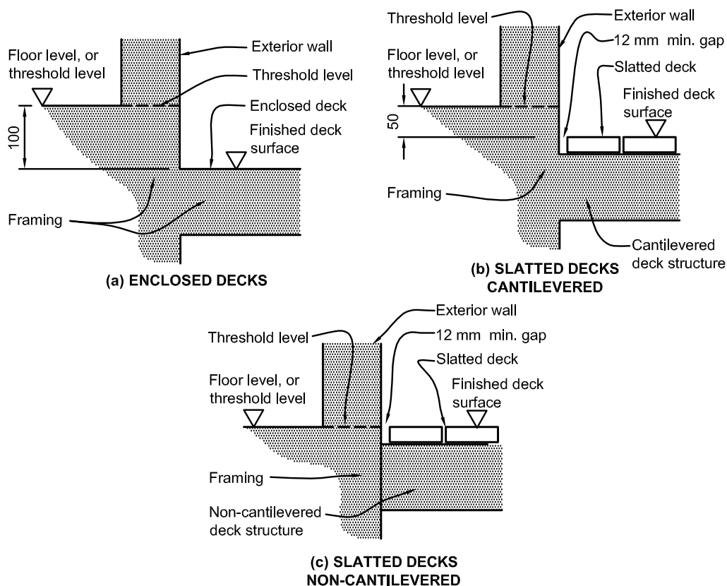
Figure 7.2.1.1: Threshold separation
