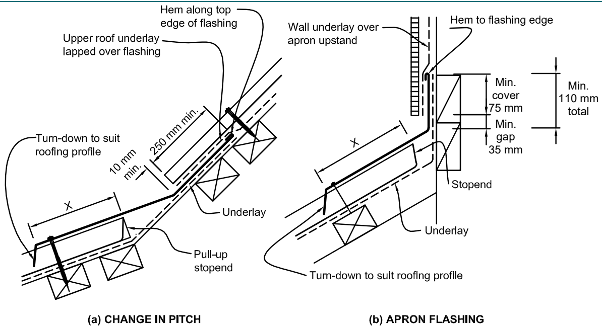
Figure 8.4.9.7B: Apron flashing and change in pitch for profiled metal
