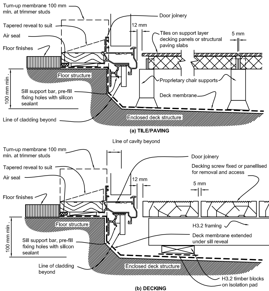
Figure 7.4.1: Level thresholds for enclosed decks
