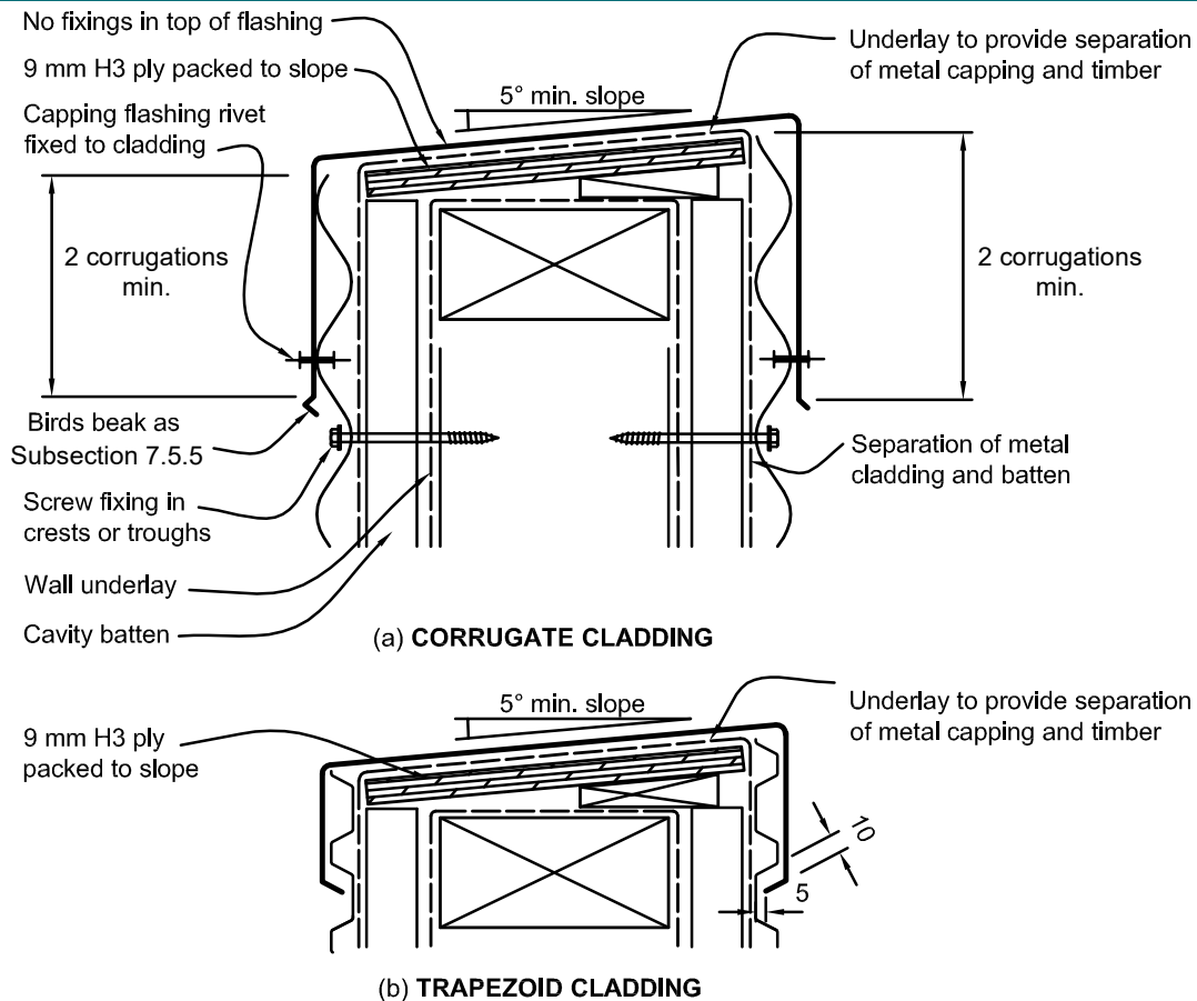
Figure 9.6.7.10: Balustrade and parapet for horizontal profiled metal
