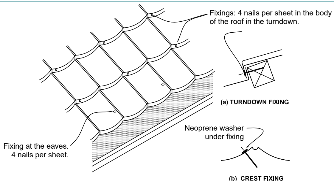
Figure 8.3.5.1: Metal tile fixings
