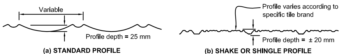
Figure 8.3.3.1: Metal tile profiles
