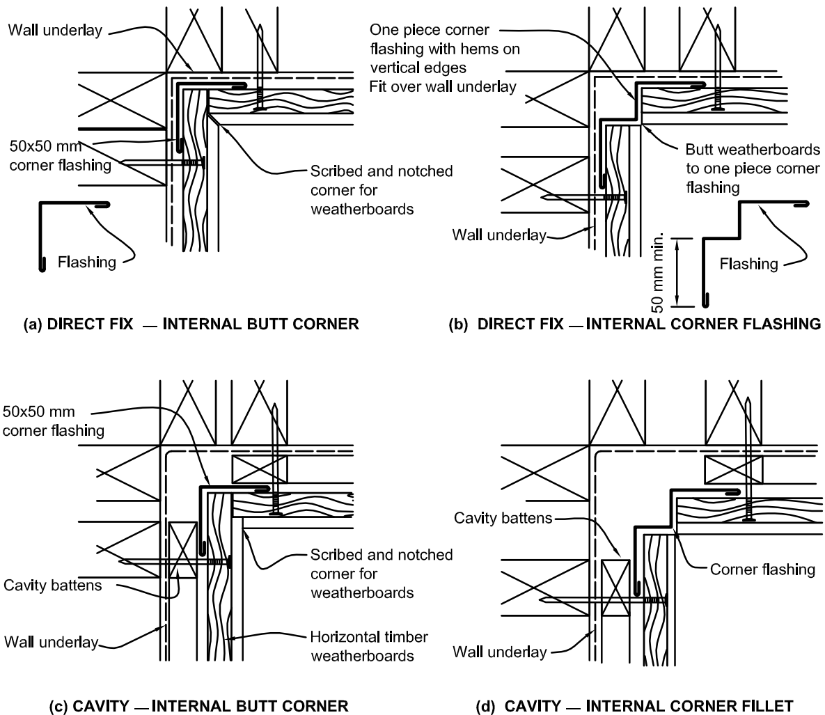
Figure 9.4.4.5: Internal corners for horizontal or vertical weatherboards
