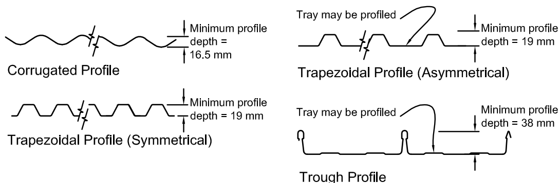
Figure 8.4.3.1: Profiled metal profiles
